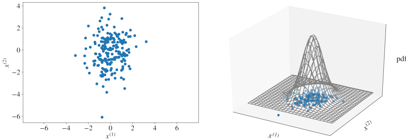
Figure 2: One-class classification solved using the one-class Gaussian method. Left: two-dimensional feature vectors. Right: the MLD curve that maximizes the likelihood of the examples on the left.
