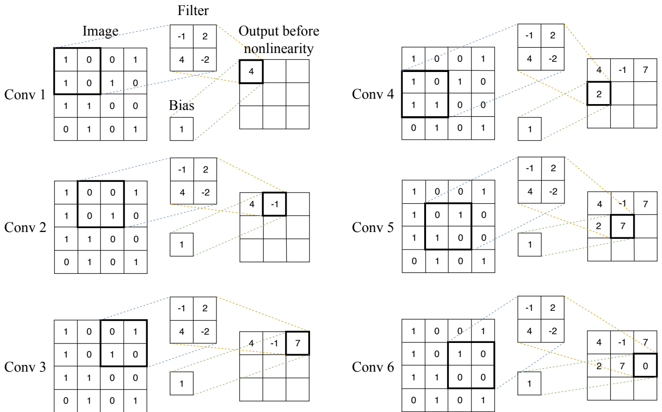
Figure 3: A filter convolving across an image.
