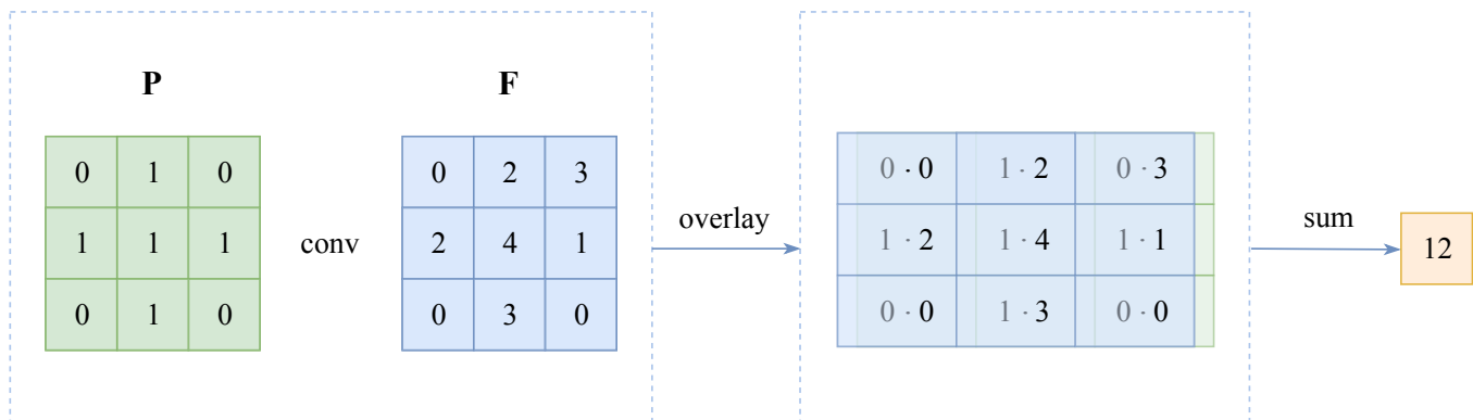
Figure 2: A convolution between two matrices.
