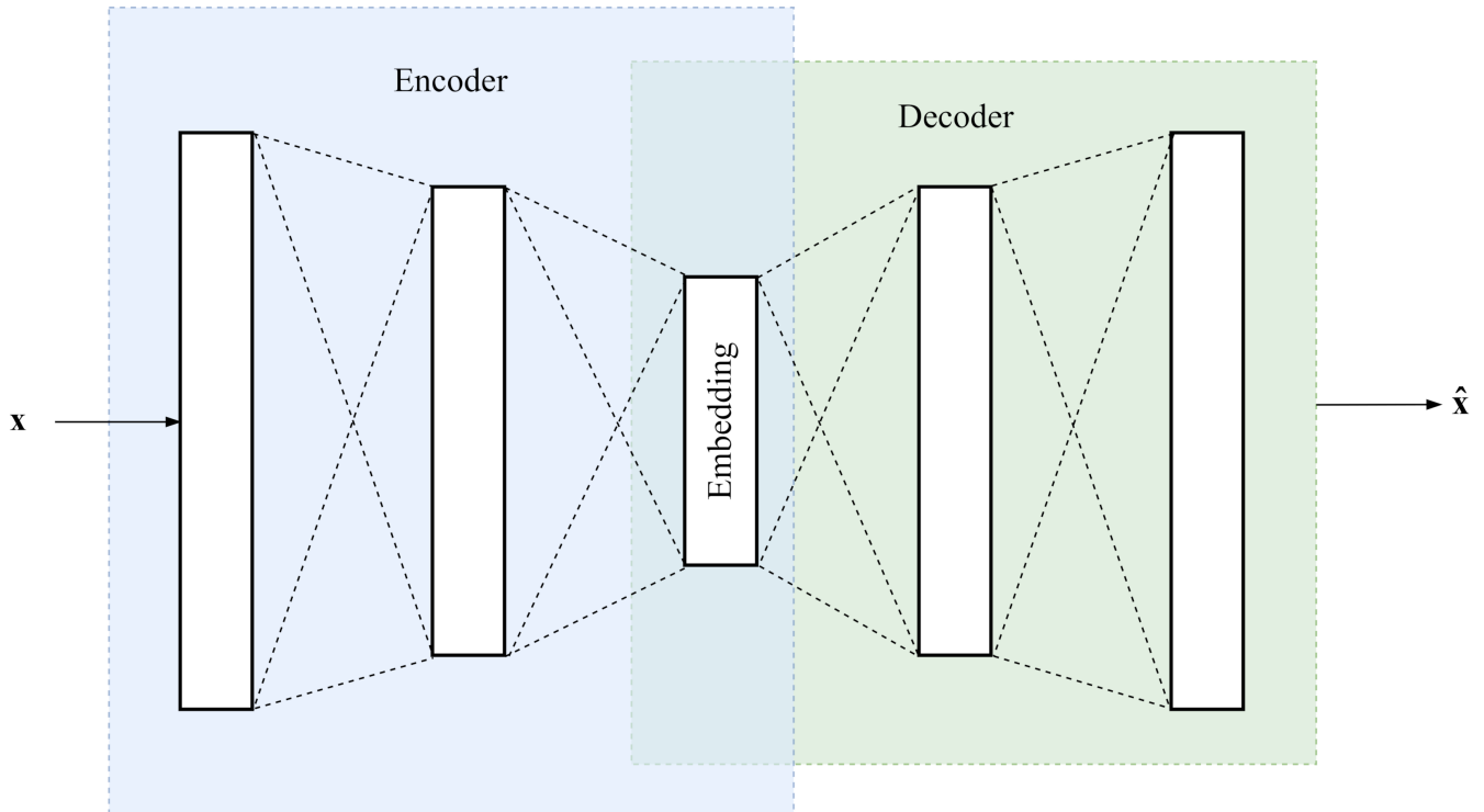
Figure 6: Autoencoder.
